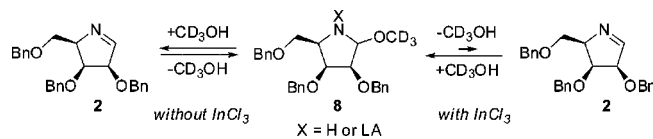
Figure 2. 13 C-APT NMR showed addition of the solvent, CD 3 OH to the imine 2 . This equilibrium between 2 and 8 shifted towards 8 when InCl 3 was added.
