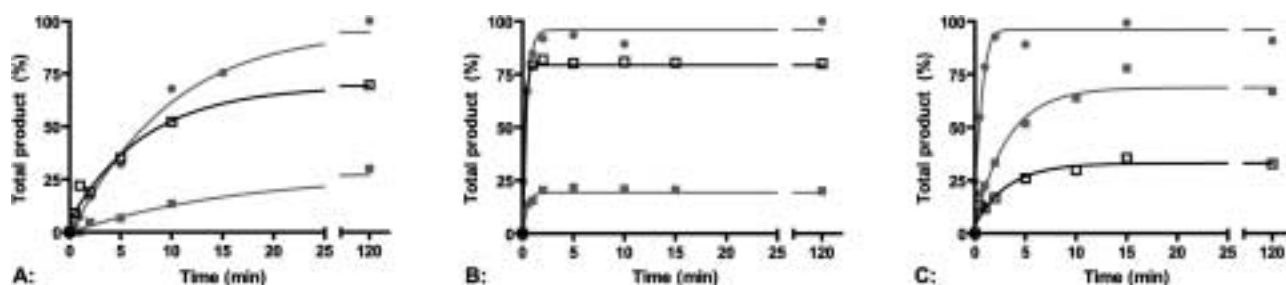
Figure 1. Formation of Ugi-3CR products over time as monitored by LC/MS. A: 1 equiv. 2,2,4,4-tetramethylbutyl isocyanide ( t MB-NC) and 1 equiv. pentanoic acid, MeOH, 0.1 M, 0 °C; B: 25 equiv. t MB-NC and 1 equiv. pentanoic acid, MeOH, 0.1 M, 0 °C. C: 1 equiv. t MB-NC and 25 equiv. pentanoic acid, MeOH, 0.1 M, 0 °C. Filled gray circles: 2,3- cis ( 3 ) formed without InCl 3 ; filled gray squares: 2,3- cis ( 3 ) formed with 1 equiv. InCl 3 ; open black squares: 2,3- trans ( 4 ) formed with 1 equiv. InCl 3 .
