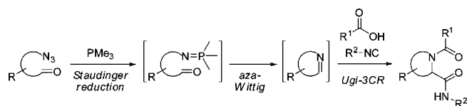
Scheme 1. Overview of the SAWU-3CR reaction sequence.
