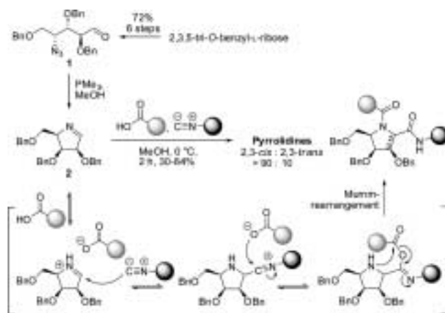
Scheme 2. Synthesis of pyrrolidines from the 4-azidoaldehyde 1 with the tandem SAWU-3CR.
