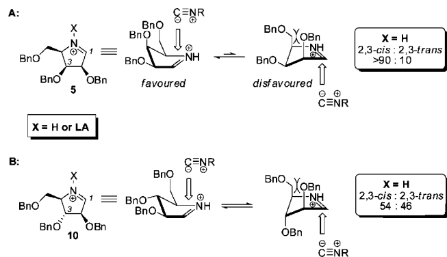
Figure 3. A: Formation of the 2,3- cis product from 5 by isocyanide attack from the concave face of the favoured conformer. B: Formation of ca. 1:1 mixture from 10 due to absence of a favoured conformer.
