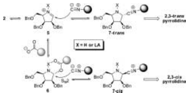
Scheme 3. Isocyanide addition via acyloxy/contact ion-pair intermediate 6 .
